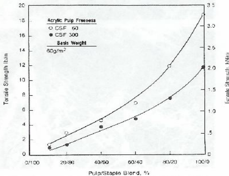
Figure 3: Tensile Strength of Acrylic Papers
